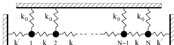
Fig. 1 A schematic description of the model
