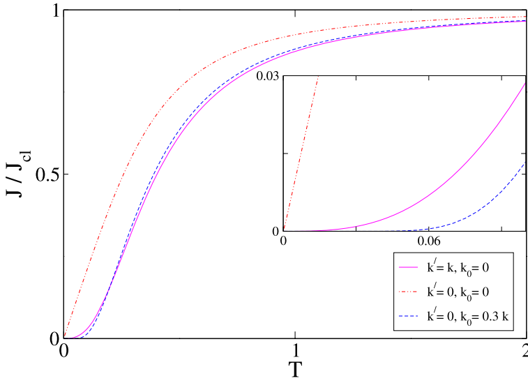
Fig. 2 Plot of the scaled heat current with temperature (in units of \hbar(k/m)^{1/2}/k_B ) for three different parameter regimes (see text). Inset shows the low temperature behavior
